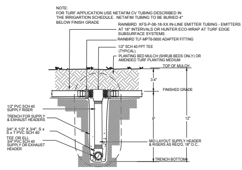
5 DRIP INTAKE HEADER MANIFOLD NTS
