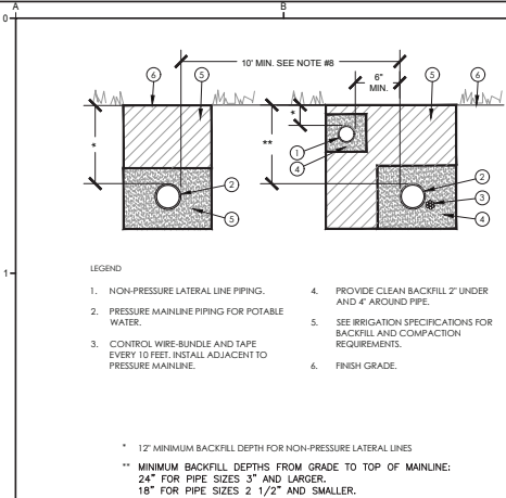
1 TRENCHING NTS
