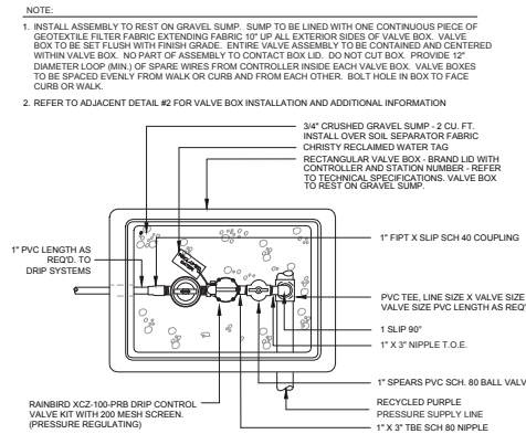
3 DRIP VALVE NTS
