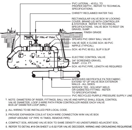
2 ELECTRIC CONTROL VALVE NTS
