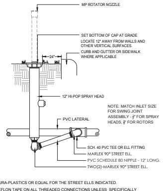
4 12" POP-UP SPRINKLER NTS
