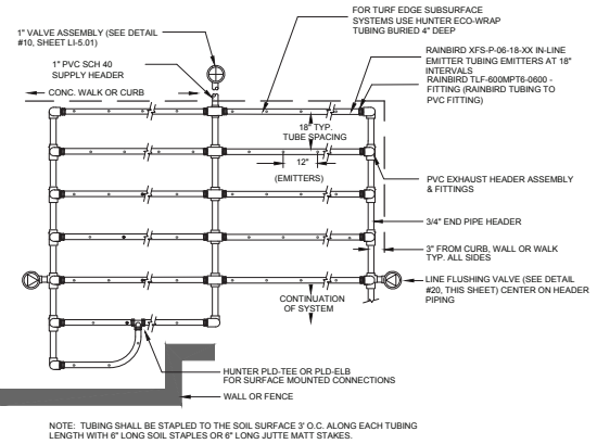
6 IN-LINE EMITTER TUBING IRRIGATION LAYOUT SHRUB DRIP CONDITION NTS
