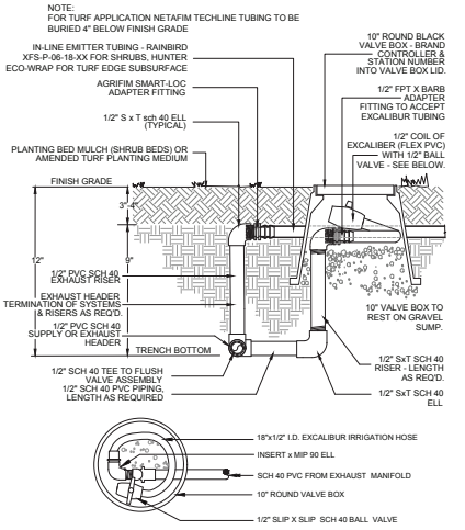
7 DRIP EXHAUST HEADER MANIFOLD - FLUSH VALVE NTS
